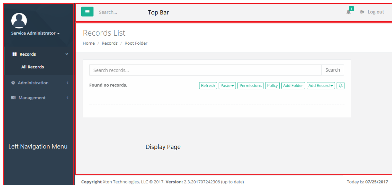
Figure 2: XTAM Graphical User Interface
